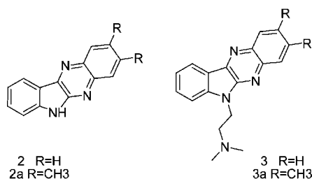
Figure 6. Left: 6 H -indolo[2,3- b ]quinoxaline, 2 , and 2,3-dimethyl-6 H -indolo[2,3- b ]quinoxaline, 2a . Right: 6-(2-dimethylaminoethyl)-6 H -indolo[2,3- b ]quinoxaline, 3 , and 2,3-dimethyl-6-(2-dimethylaminoethyl)-6 H -indolo[2,3- b ]quinoxaline, 3a .
