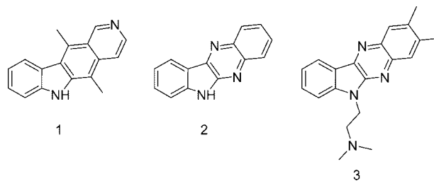
Figure 1. The alkaloid ellipticine, 1 , the indolo[2,3- b ]quinoxaline system, 2 , and the parent compound of the indoloquinoxaline derivatives used in this study: 2,3-dimethyl-6(2-dimethylaminoethyl)6 H -indolo-(2,3- b )quinoxaline (B-220), 3 .
